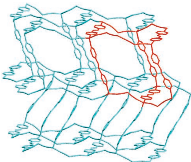
Fig. 7 One diamond-like net in the structure of \beta -Cu(dca)(bpe) 6 , with a single adamantane highlighted. Ranges for selected bond lengths and angles: Cu–N(bpe) 2.042(5)–2.125(5), Cu–N(dca) 1.915(5)–2.026(5) Å, Cu–N–C(dca) 150.5(5)–173.6(5)°.
