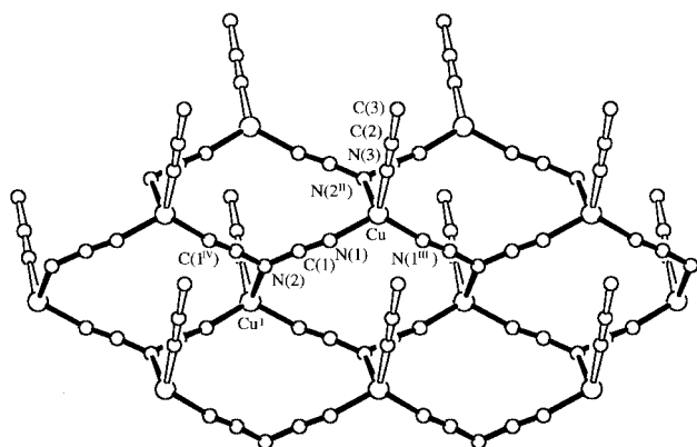
Fig. 1 A single (6,3) sheet in the structure of \text{Cu}(\text{dca})(\text{MeCN}) 1 , with terminal acetonitrile ligands represented by the open bonds. Selected bond lengths and angles: \text{Cu}-\text{N}(1) 1.942(1), \text{Cu}-\text{N}(2') 2.273(2), \text{Cu}-\text{N}(3) 1.967(2) Å, \text{Cu}-\text{N}(1)-\text{C}(1) 168.7(1), \text{Cu}^{\text{I}}-\text{N}(2)-\text{C}(1) 118.33(9), \text{Cu}-\text{N}(3)-\text{C}(2) 175.0(2)°.
