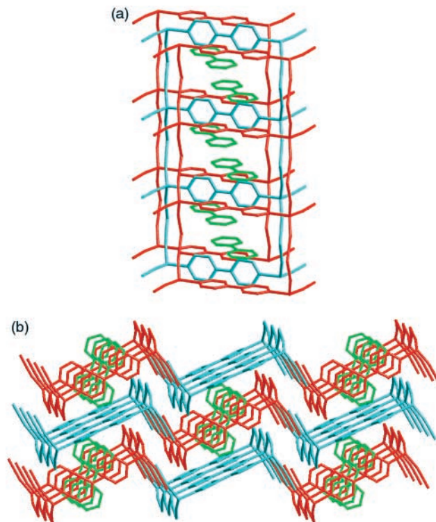
Fig. 3 (a) Intercalation of guest \text{bipy} molecules (green) in a single stack of ladders in the structure of \text{Cu}_2(\text{dca})_2(\text{bipy})(\text{MeCN})_2 \cdot 0.5\text{bipy} 3 . The \text{bipy} guests lie in the windows of one type of ladder (red), and these ladders stack in an alternating fashion with a second type of ladder (blue). Selected bond lengths and angles for red ladders (blue ladders in parentheses): \text{Cu}-\text{N}(\text{bipy}) 2.090(5) (2.088(5)), \text{Cu}-\text{N}(\text{MeCN}) 2.004(4) (1.977(5)), \text{Cu}-\text{N}(\text{dca}) 1.971(3) Å (1.976(4) Å), \text{Cu}-\text{N}-\text{C}(\text{dca}) 168.3(3)° (169.7(4)°). (b) Interdigitation of adjacent stacks of ladders in 3 .
