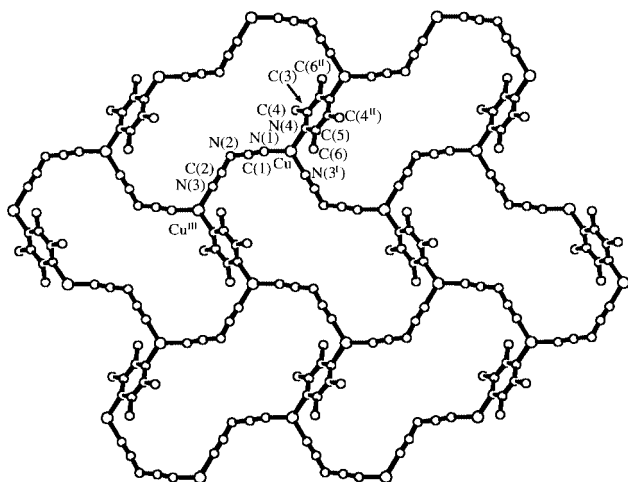
Fig. 2 A single (6,3) sheet in the structure of \text{Cu}(\text{dca})(\text{Me}_4\text{pyz})_{1/2} ( 2 ). Selected bond lengths and angles: \text{Cu}-\text{N}(4) 2.005(2), \text{Cu}-\text{N}(1) 1.911(2), \text{Cu}-\text{N}(3') 1.931(2) Å, \text{Cu}-\text{N}(1)-\text{C}(1) 169.2(2), \text{Cu}-\text{N}(3')-\text{C}(2') 176.4(2)°.
